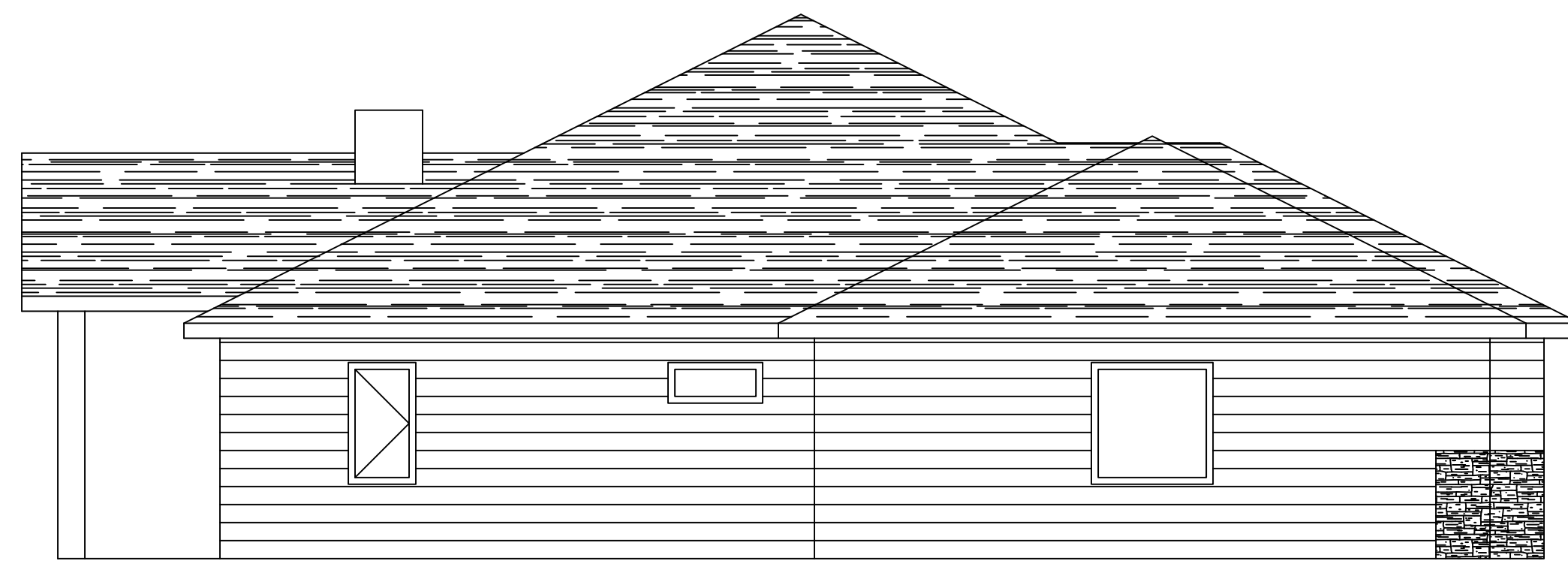
LEFT ELEVATION SCALE: 3/16"=1'-0"
