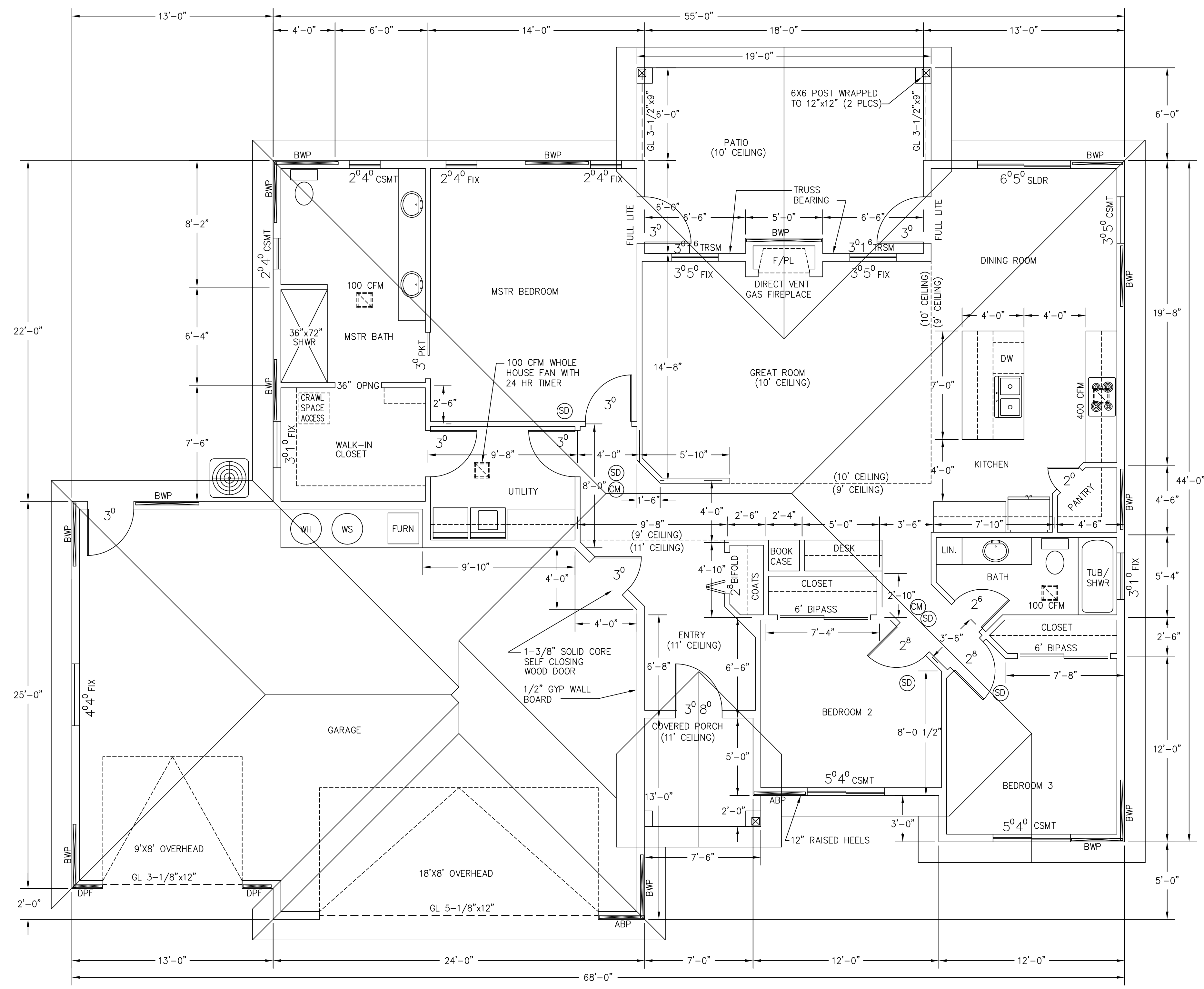
FLOOR PLAN SCALE: 1/4"=1'-0" (9' CEILING, UNLESS NOTED OTHERWISE)
