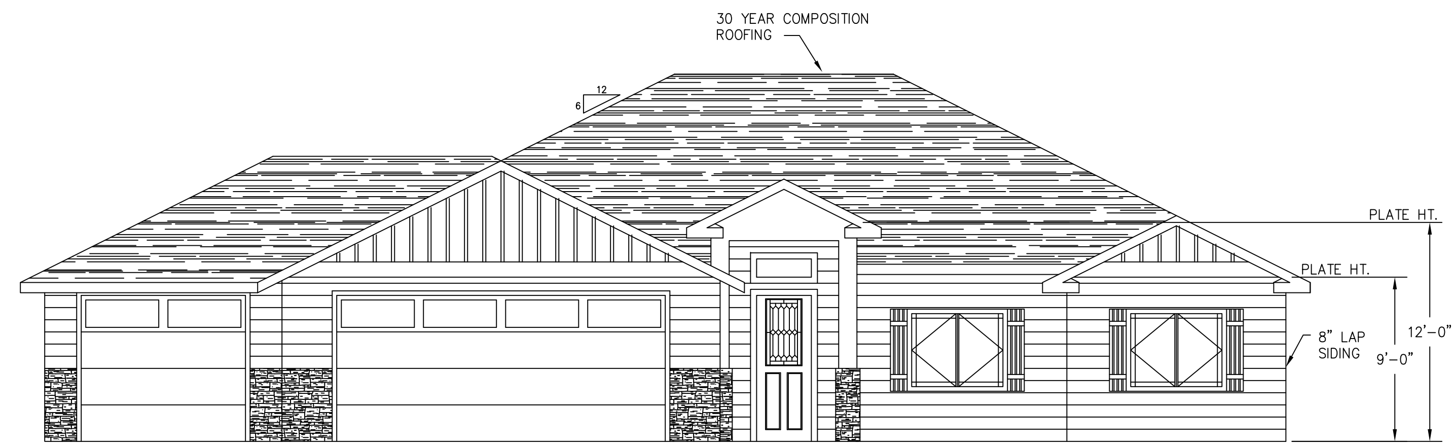
FRONT ELEVATION SCALE: 3/16"=1'-0"
